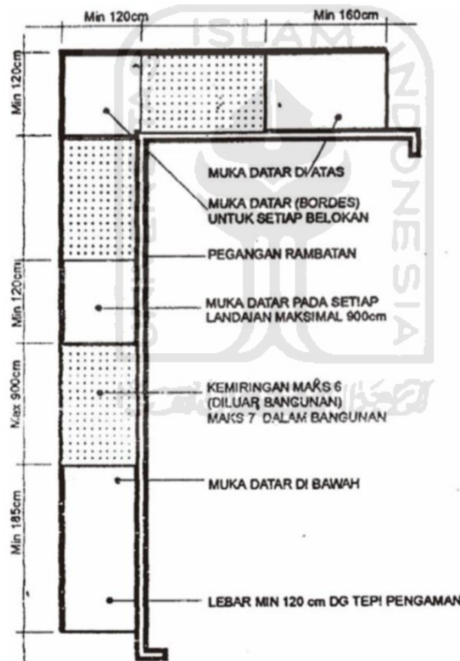
Gambar 3.10 Tipikal Ramp
