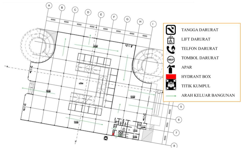
Gambar 5.26 Fire Protection
