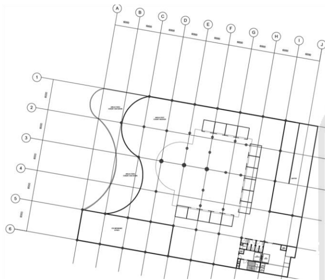
Gambar 4.1 Denah Basement
