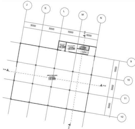
Gambar 5.5 Denah Massa Dua Ground Floor
