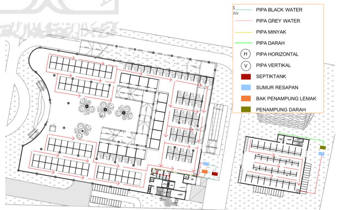
Gambar 4.14 Sistem Air Kotor
