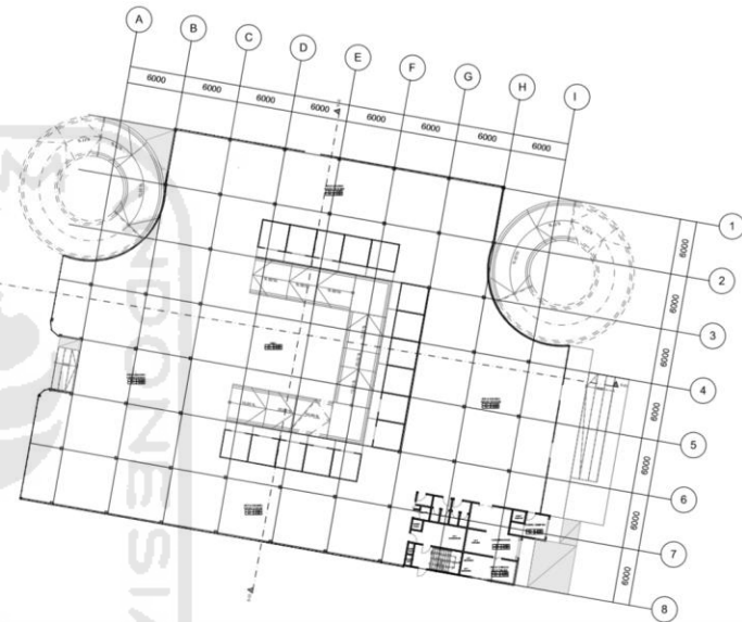
Gambar 5.2 Denah Utama Ground Floor
