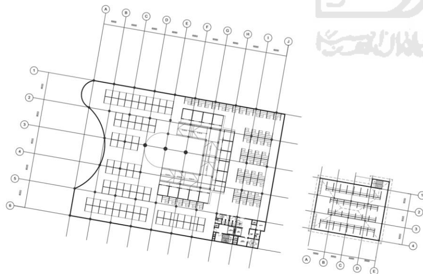
Gambar 4.3 Denah Lantai 2
