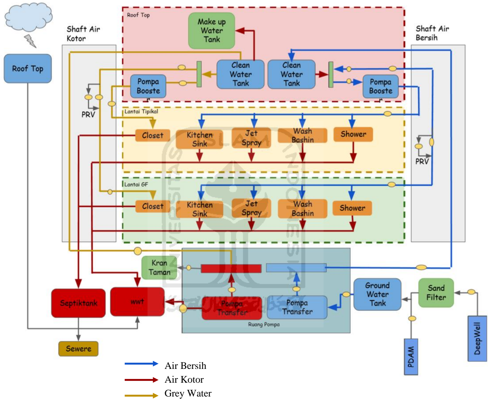
Gambar 3.9 Distribusi Air Kotor
