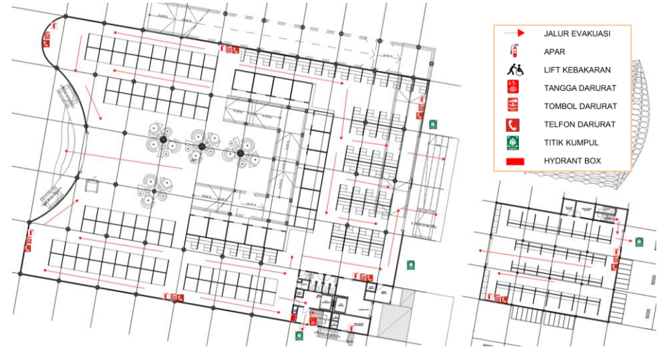
Gambar 4.16 Fire Protection
