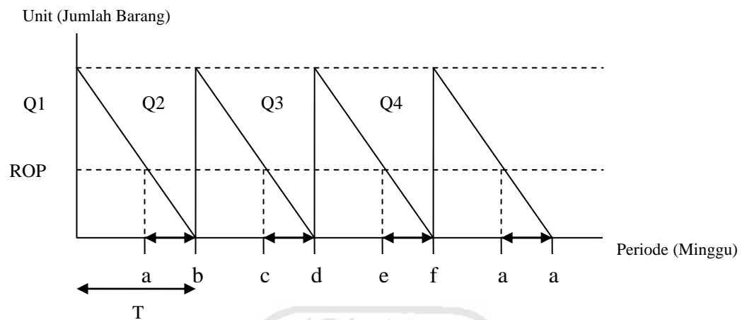
Gambar 2.5. Model inventori klasik (EOQ)
