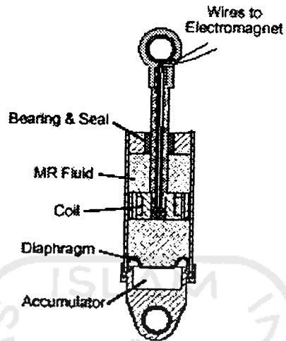
Gambar 2.1 Skema MR Damper (Spencer dan kawan-kawan, 1996)
