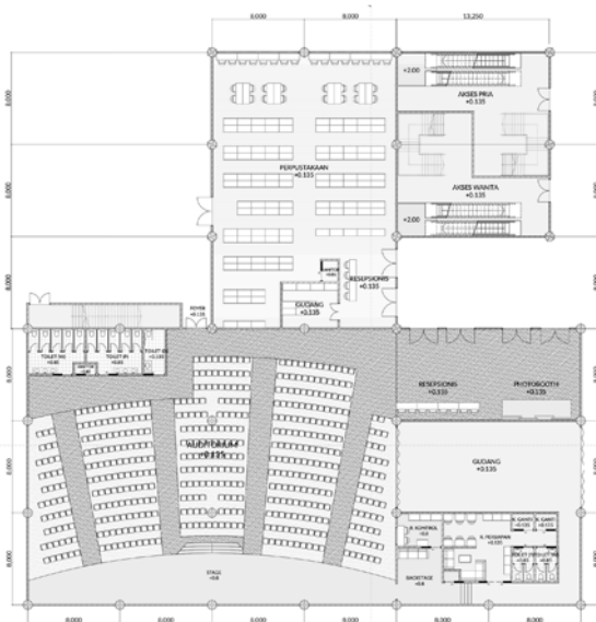
Gambar 109. Denah It. 1 alternatif desain 01 Sumber : Hernanta, 2020
