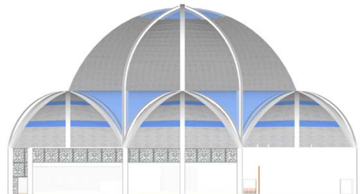
TAMPAK KIRI
