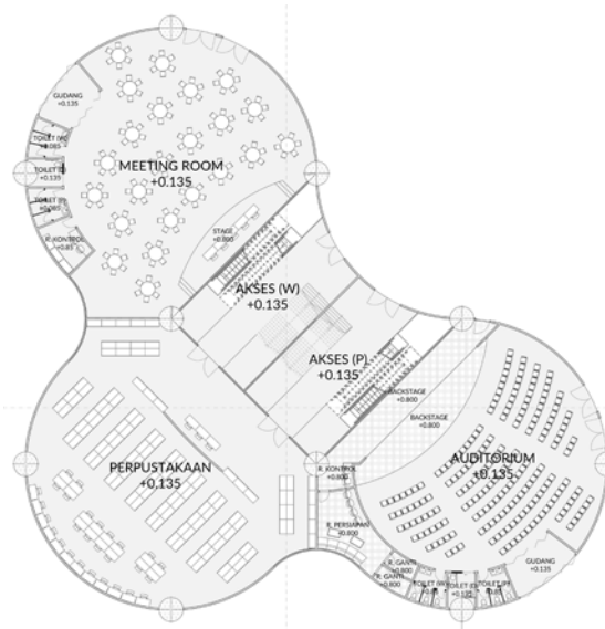
Gambar 110. Denah It. 1 alternatif desain 02 Sumber : Hernanta, 2020
