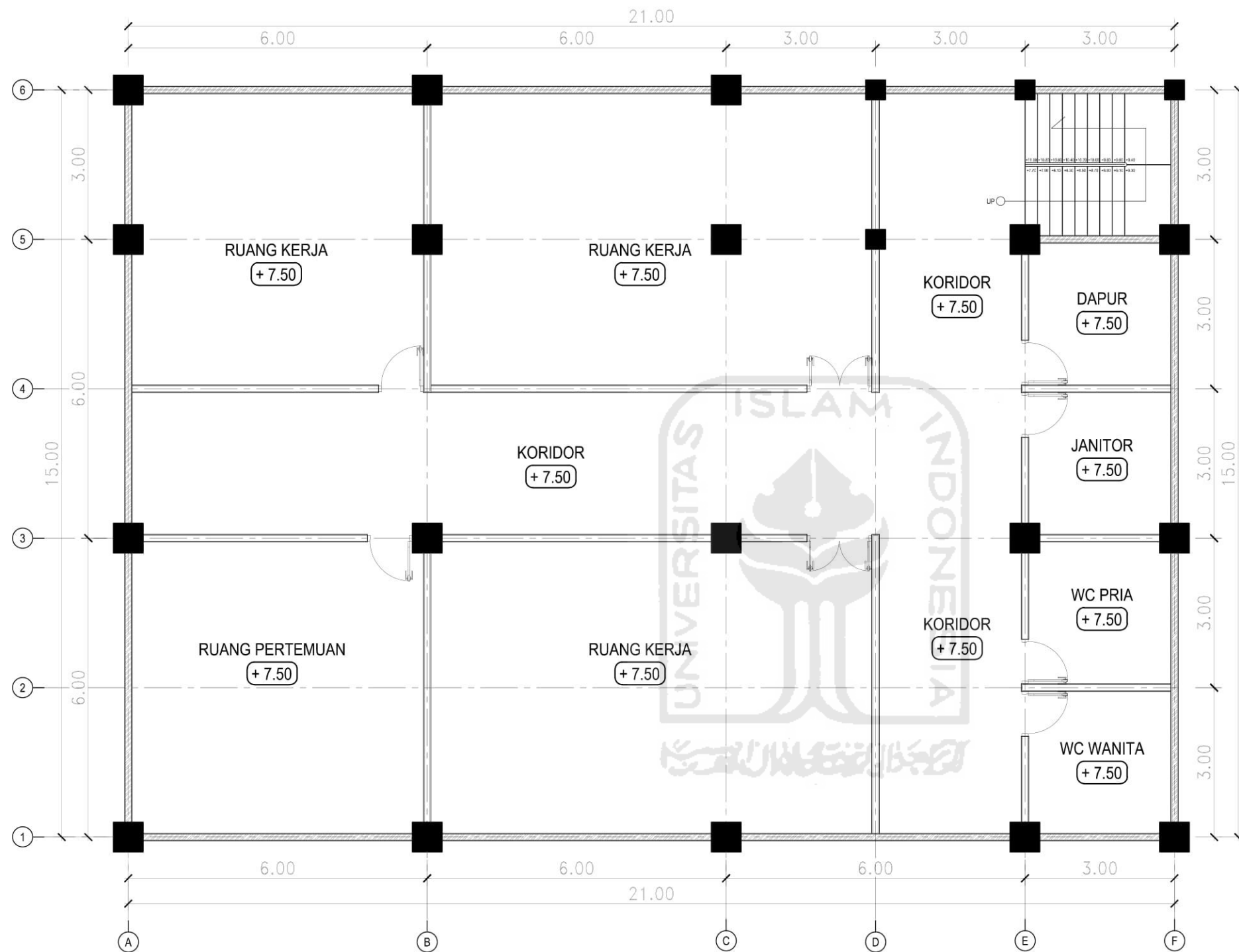
DENAH LANTAI 3 1:100
