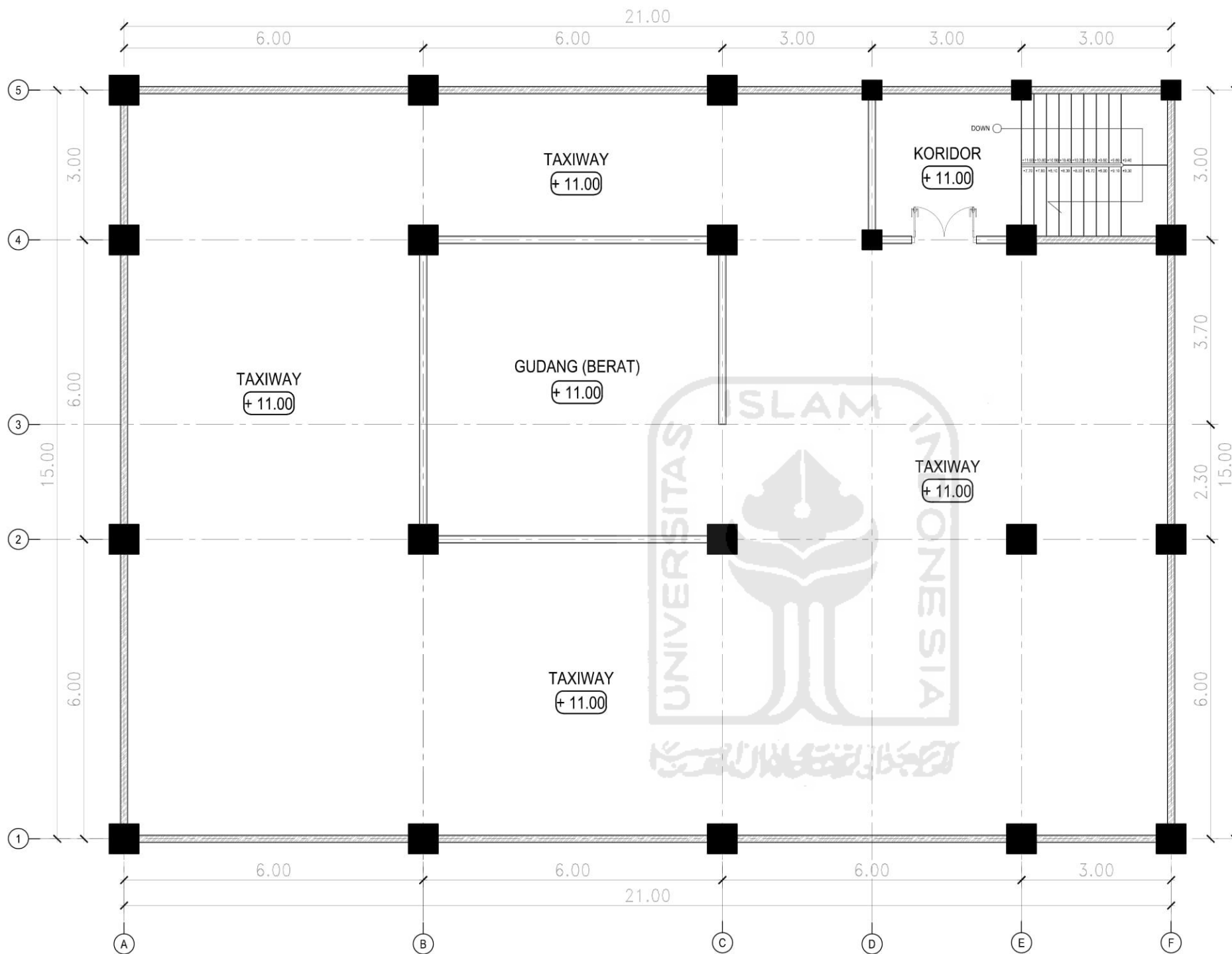
DENAH LANTAI 4 1:100
