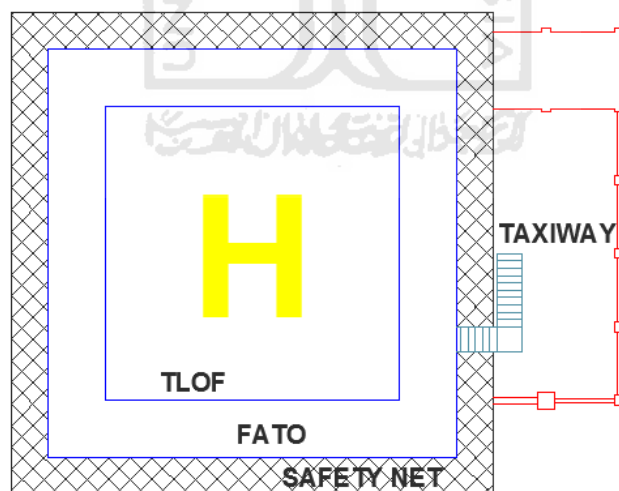
Gambar 3.11 Bagian-bagian Helipad
