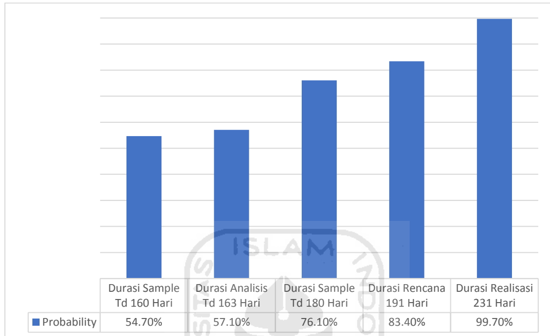
Gambar 5.12 Diagram Probability
