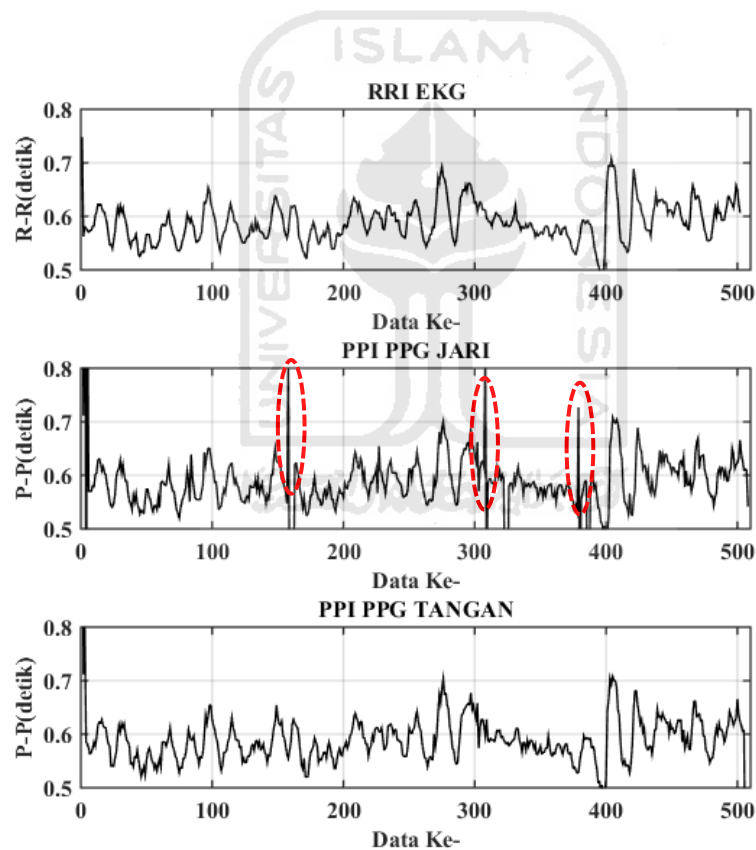
Gambar 4.3 Contoh Miss Detection ketika deteksi Peak
