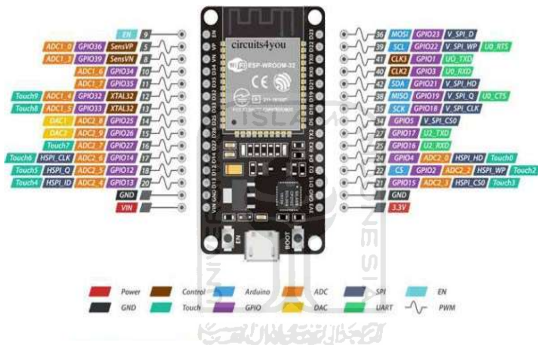
Gambar 2.9 Pinout NodeMcu
