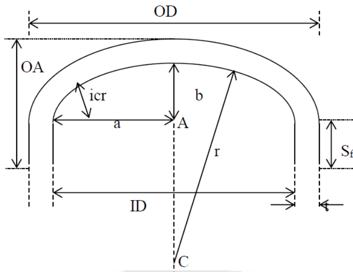
Gambar 3 Head reactor
