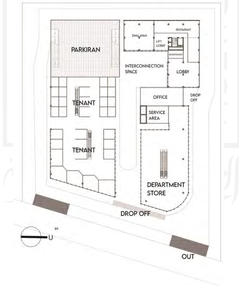
Gambar 4.4 Denah Lantai Dasar
