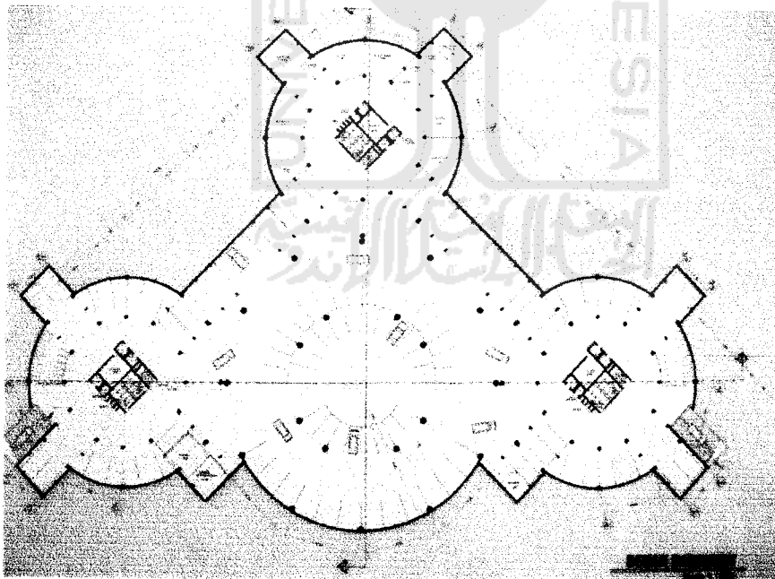
Denah Basement
