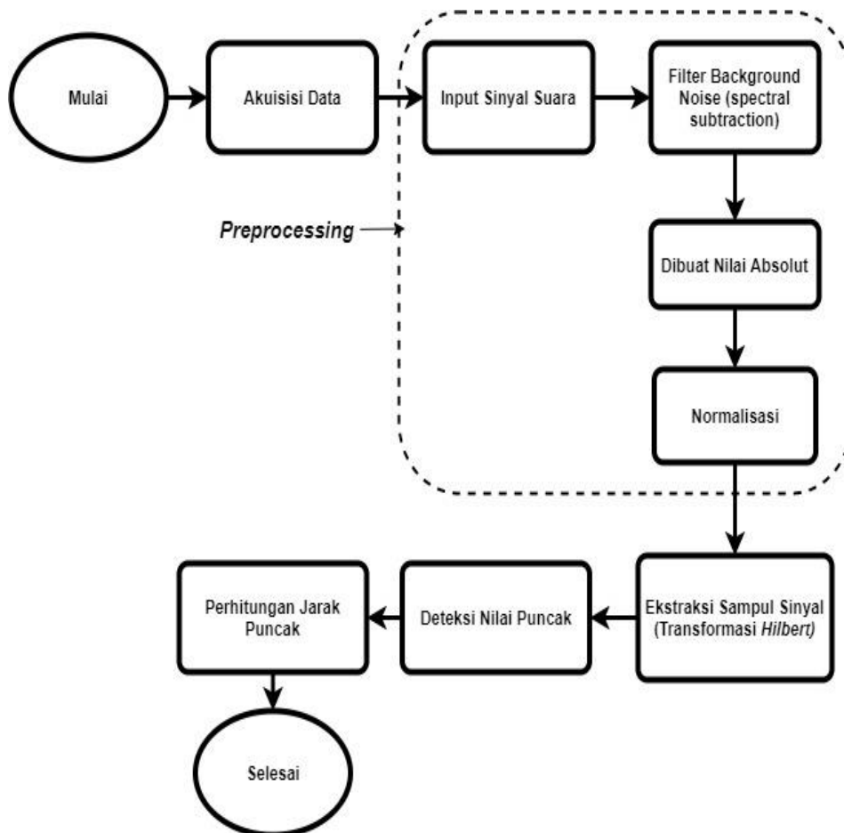
Gambar 3.1 Alur penelitian
