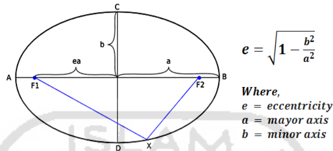
Gambar 2.11 Perhitungan Eccentricity
