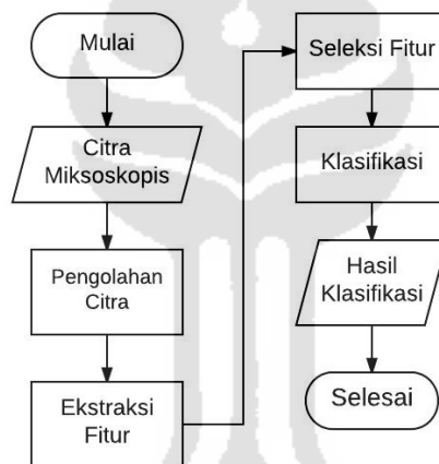
Gambar 4.1 Flowchart Sistem
