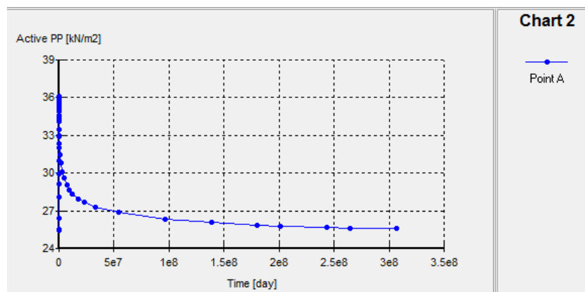
Gambar L-11.9 Kurva Time vs Pore Pressure Timbunan 3 m, Tanah Asli 70 m
