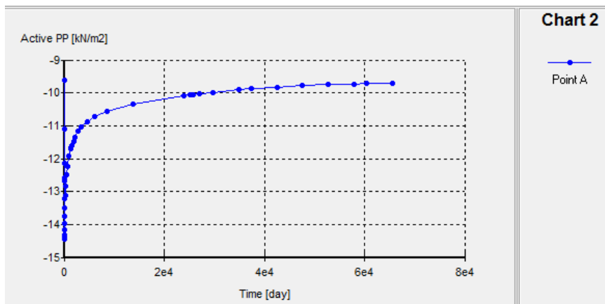
Gambar L-11.5 Kurva Time vs Pore Pressure Timbunan 2 m, Tanah Asli 35 m
