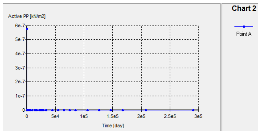
Gambar L-11.6 Kurva Time vs Pore Pressure Timbunan 2 m, Tanah Asli 70 m
