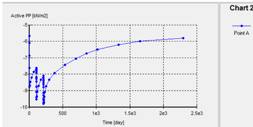
Gambar L-11.7 Kurva Time vs Pore Pressure Timbunan 3 m, Tanah Asli 5 m
