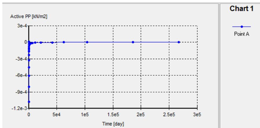
Gambar L-11.3 Kurva Time vs Pore Pressure Timbunan 1 m, Tanah Asli 70 m
