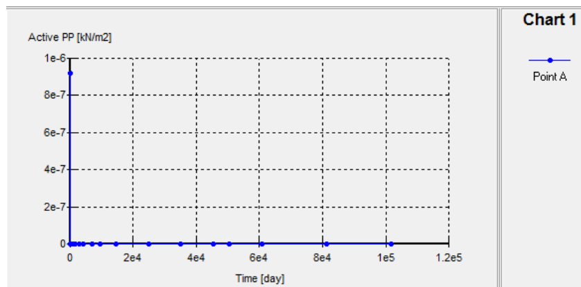
Gambar L-11.8 Kurva Time vs Pore Pressure Timbunan 3 m, Tanah Asli 35 m
