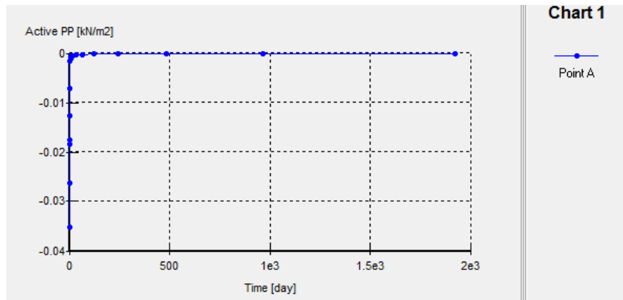
Gambar L-11.1 Kurva Time vs Pore Pressure Timbunan 1 m, Tanah Asli 5 m
