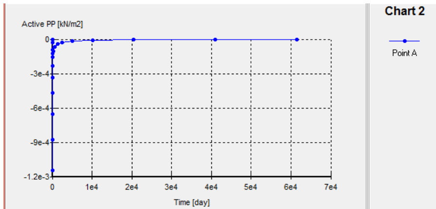
Gambar L-11.2 Kurva Time vs Pore Pressure Timbunan 1 m, Tanah Asli 35 m
