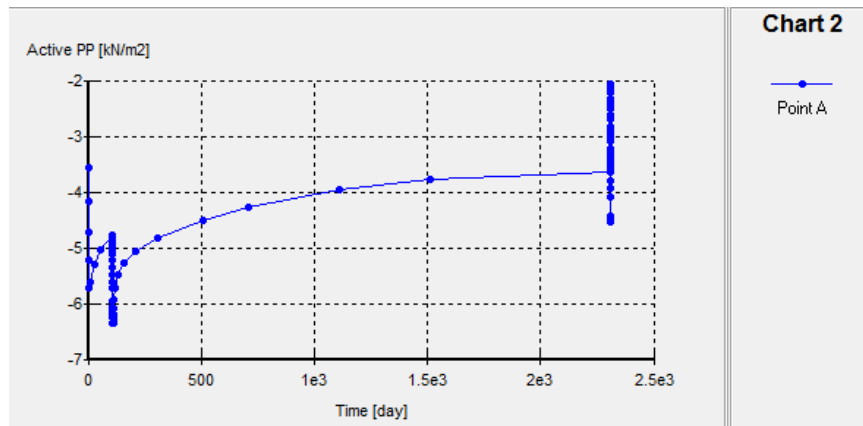
Gambar L-11.4 Kurva Time vs Pore Pressure Timbunan 2 m, Tanah Asli 5 m
