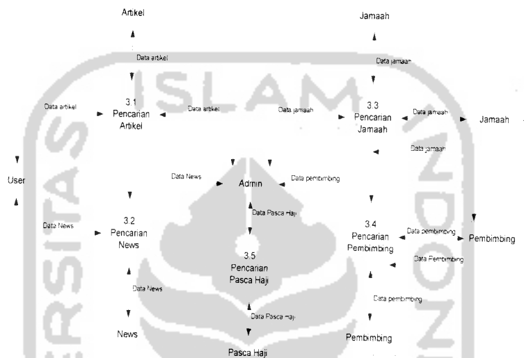
Gambar 3.5 DFD Level 2 proses pencarian
