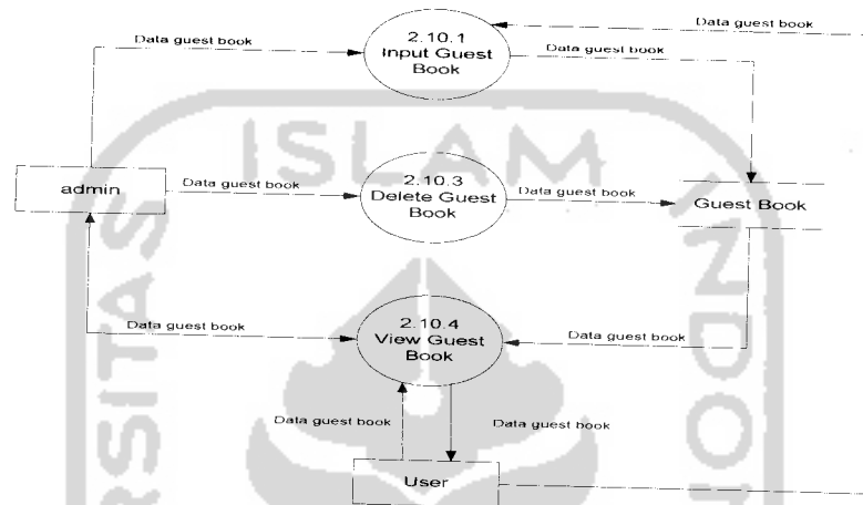
Gambar 3.15 DFD Level 3 proses manajemen data guest book
