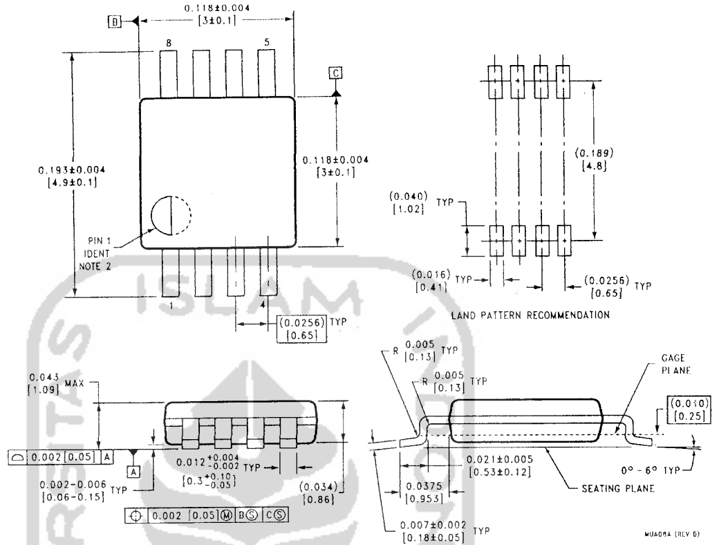
8-Lead (0.118" Wide) Molded Mini Small Outline Package Order Number LM385MM-1 NS Package Number MUA08A
