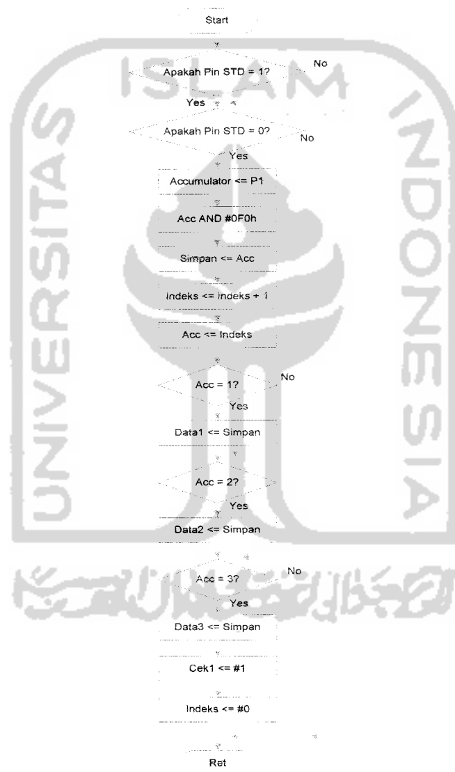
Gambar 3.11. Flowchart subroutin cek_Hp
