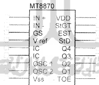
Gambar 2.3. Pin MT 8870
