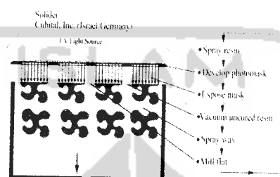
Gambar 2.6 Metode solid ground curing
