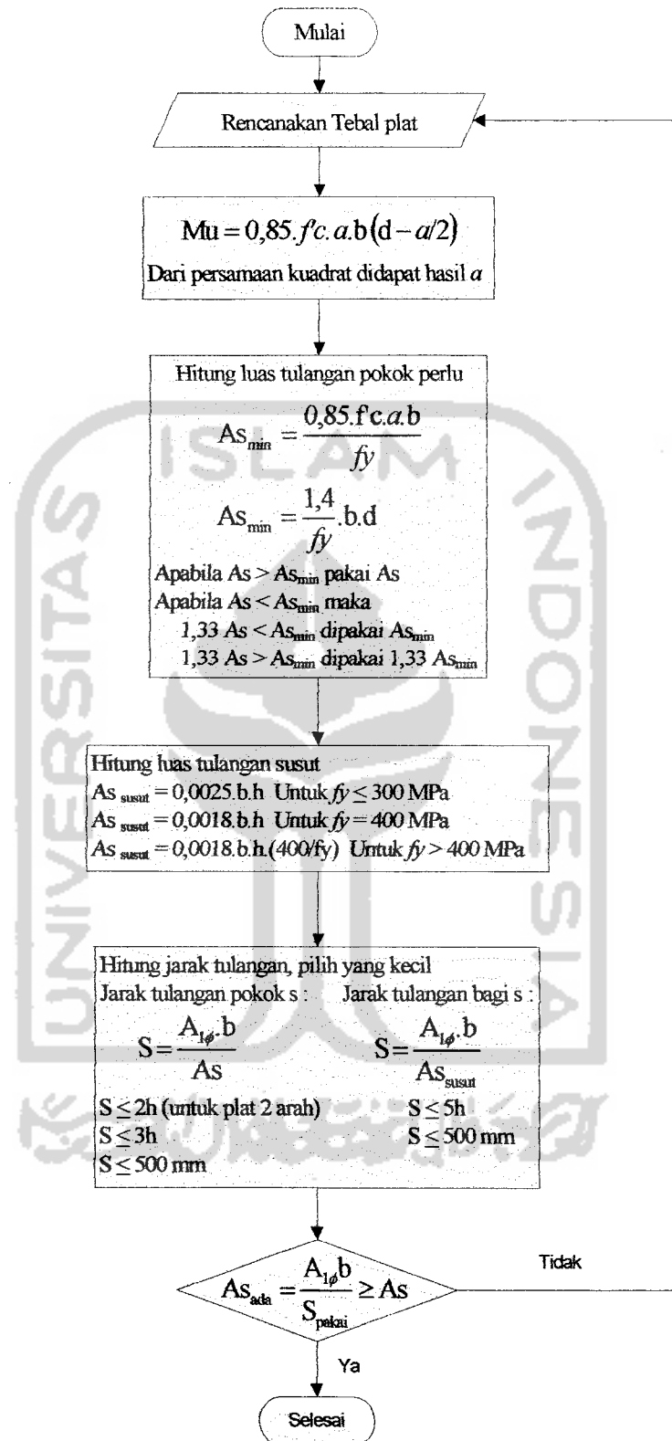
Gambar 3.3 Flow Chart Perhitungan Plat
