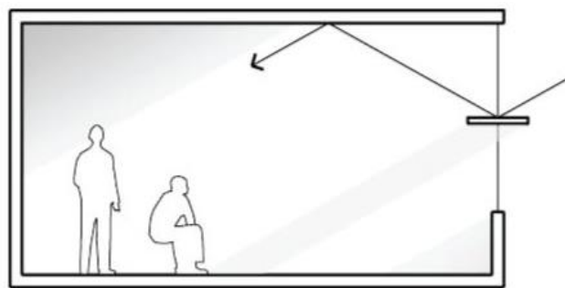
LIGHT SHELF
