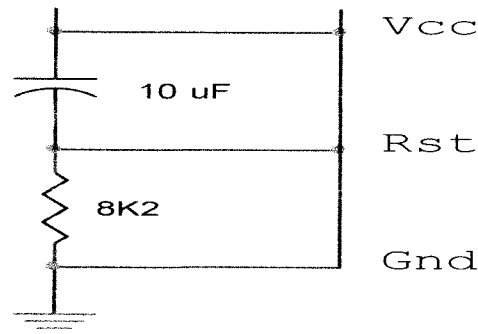
Gambar 3. 11 Rangkaian Power on Reset
