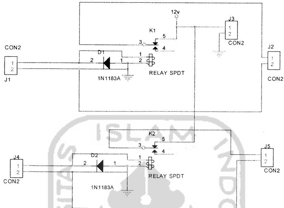
Gambar 3.13 Driver Relay
