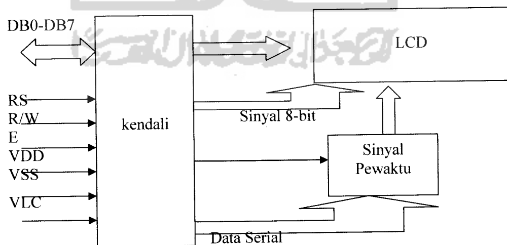
Gambar 2. 12 Blok diagram LCD
