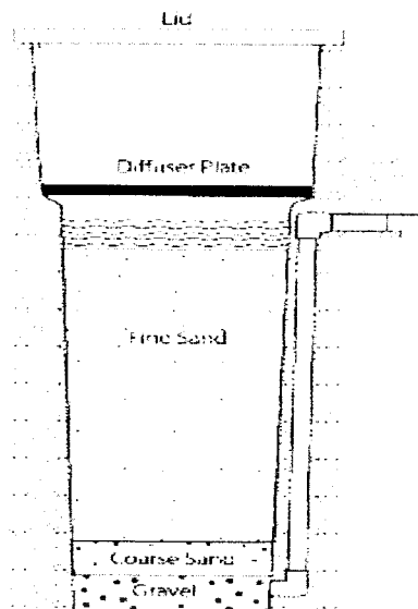
Gambar 2.1 Unit Biosand Filter
