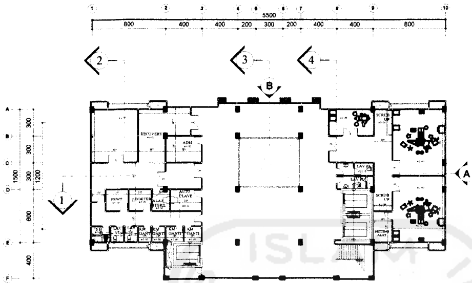
DENAH LANTAI 1
