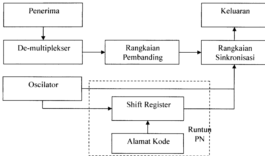
Gambar 3.1 Untai penerima
