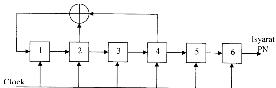
Gambar 2.6 Diagram blok register geser
