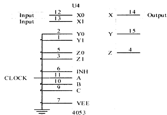
Gambar 3.6 Multiplekser analog
