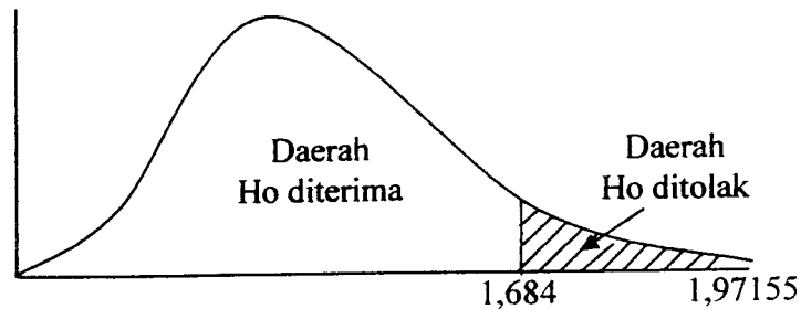
Gambar 6.4 Kurva Uji t Dummy
