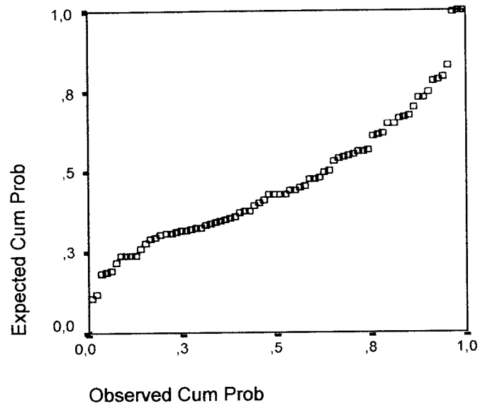
Normal P-P Plot of Regression Standardized Dependent Variable: Return
