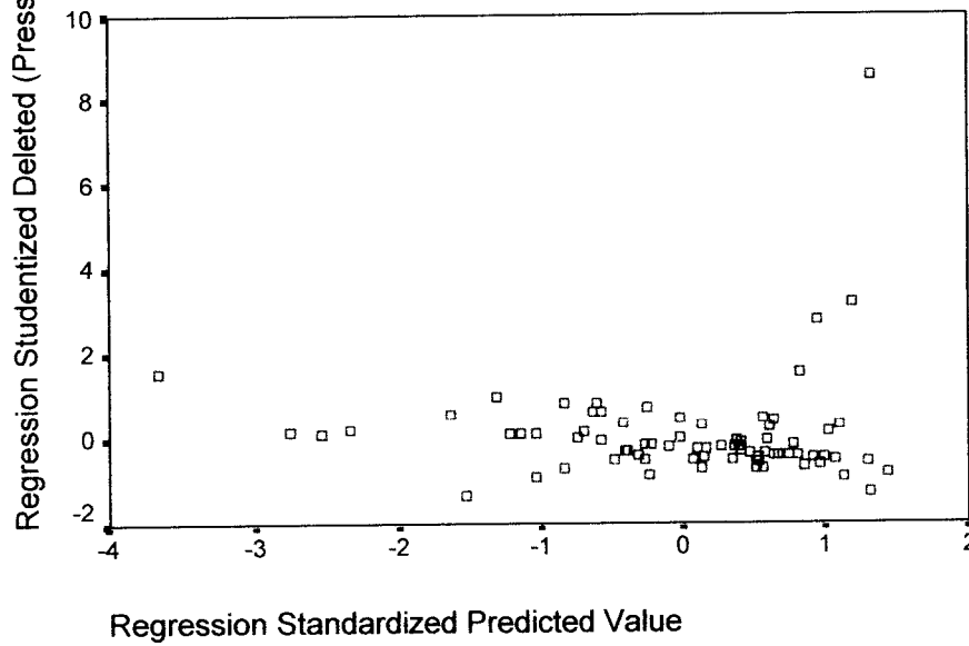
Scatterplot Dependent Variable: Return
