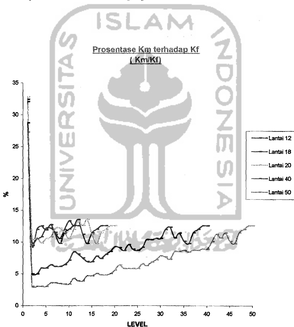
Gambar 5.1 Prosentase K_m terhadap K_f
