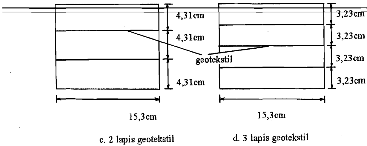
Gambar 5.5 Benda uji CBR.
