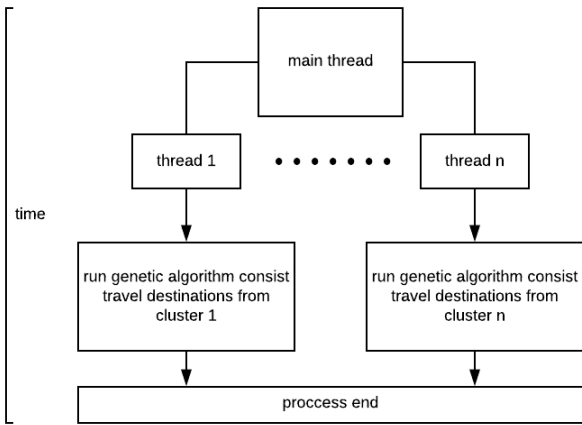
Figure 3. Multithreading Implementation
