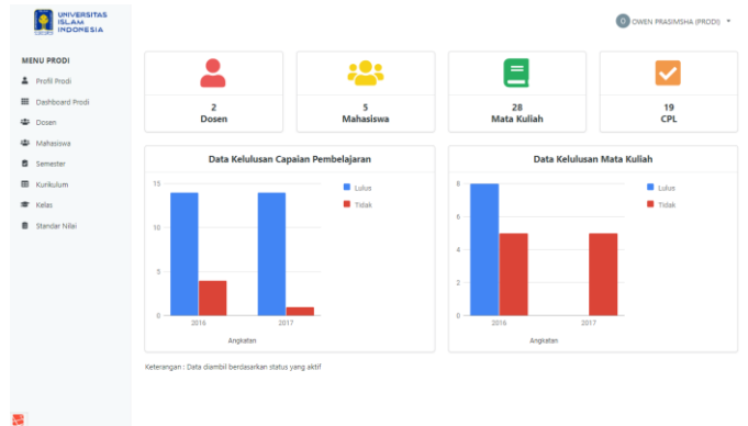
Gambar 4. 5 Halaman Dashboard
