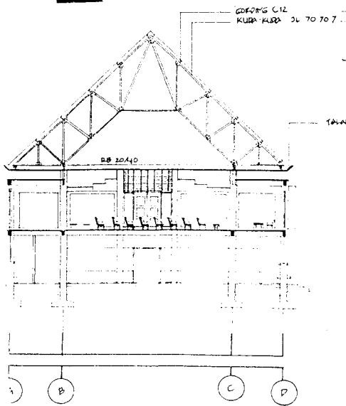
POTONGAN AUDITORIUM POT. AA
