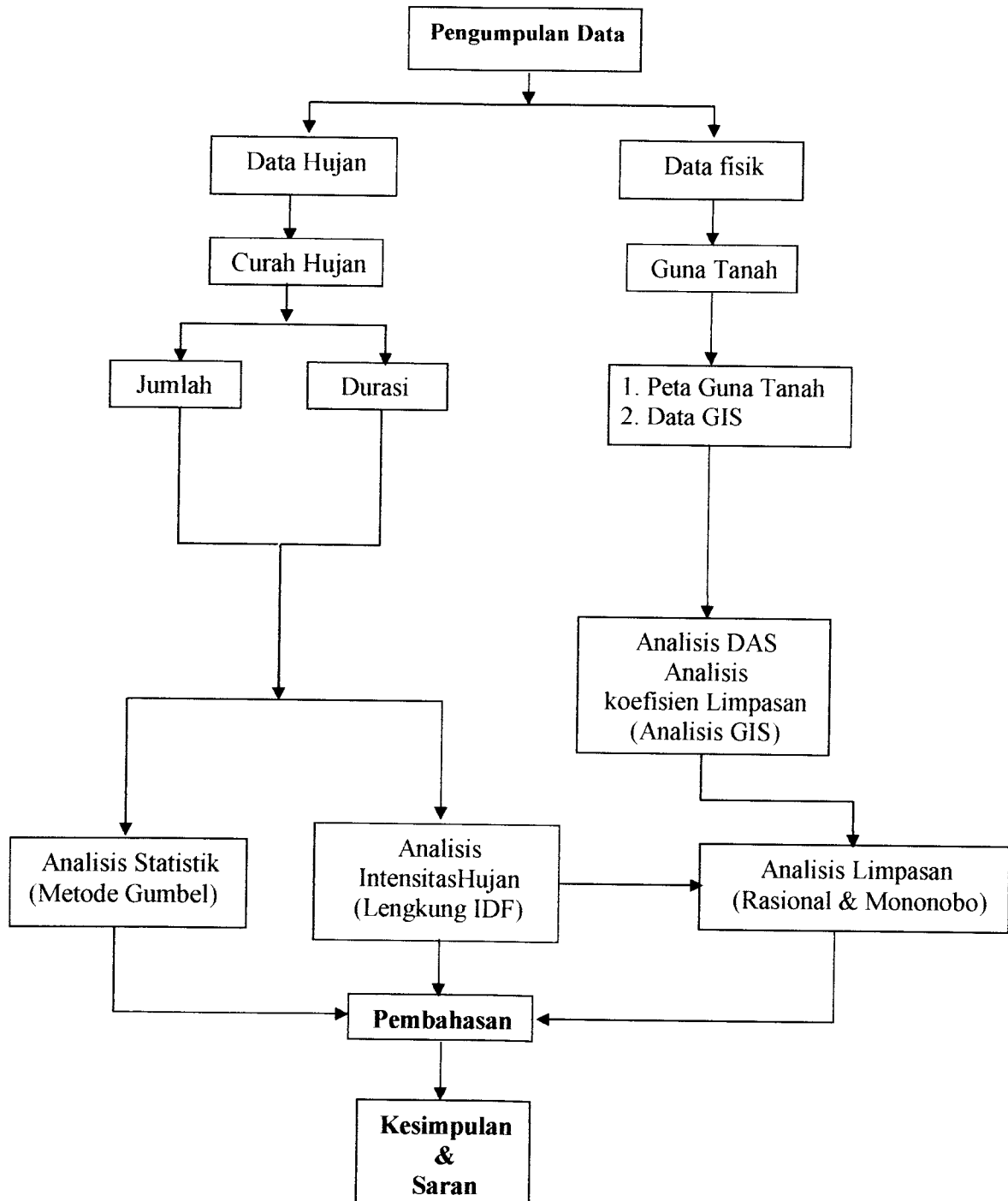
Gambar 4.1 Proses penelitian
