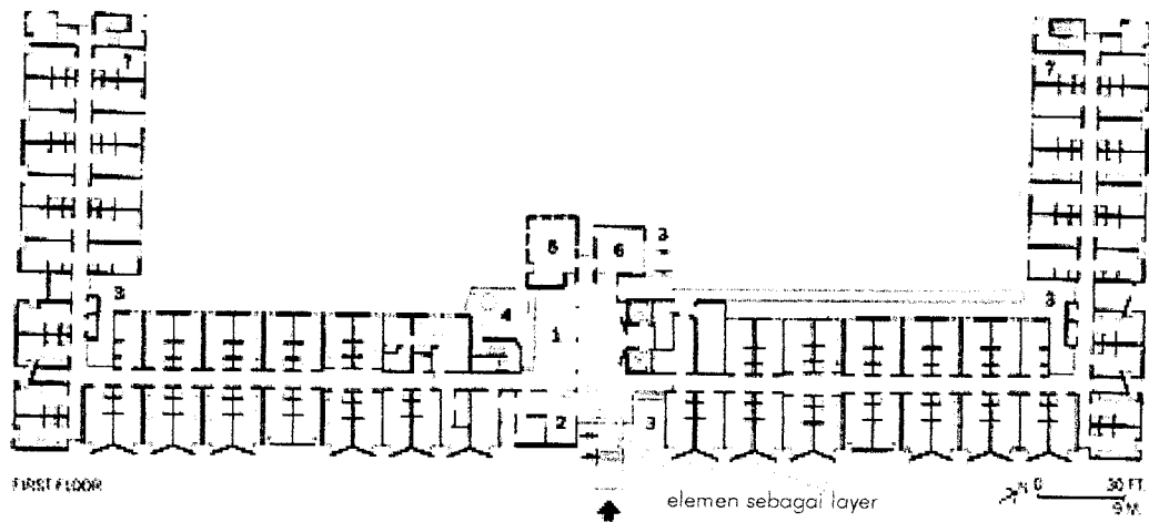
Denah Lantai 1
