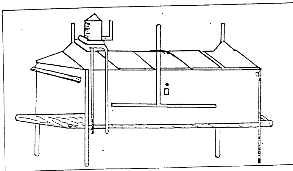
Gambar 6. Exhaust Box
