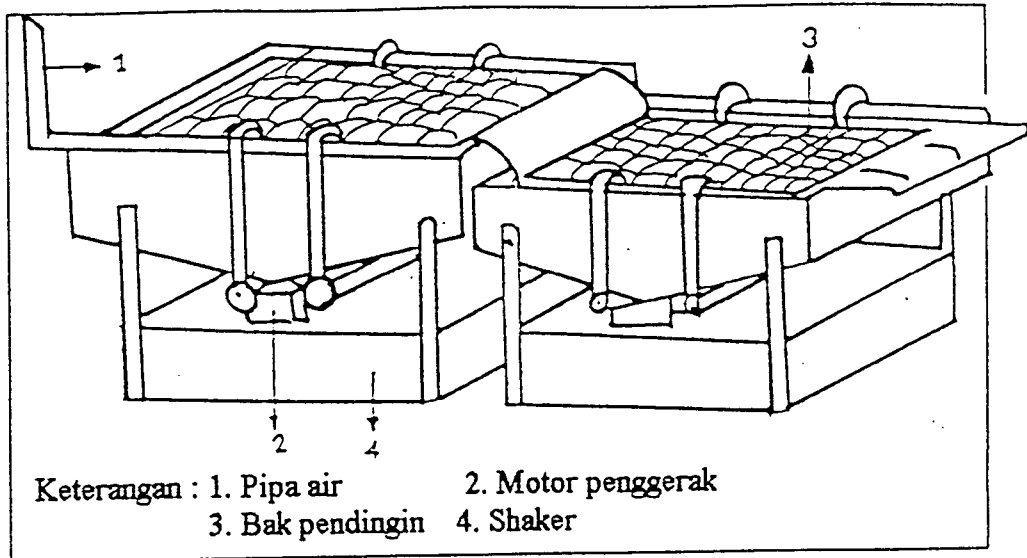
Gambar 3. Cooling Shaker
