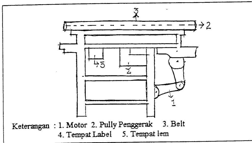
Gambar 14. Labelling Machine
