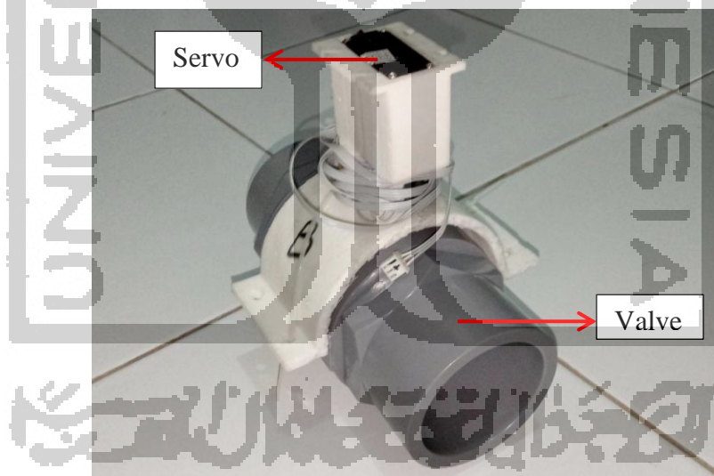
Gambar 4-4 Package Aktuator
