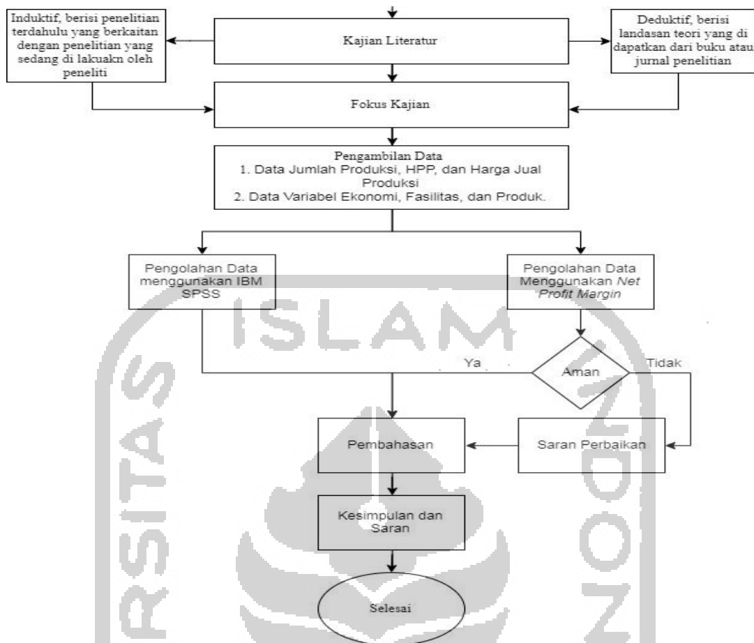
Gambar 3. 1 Alur Penelitian
