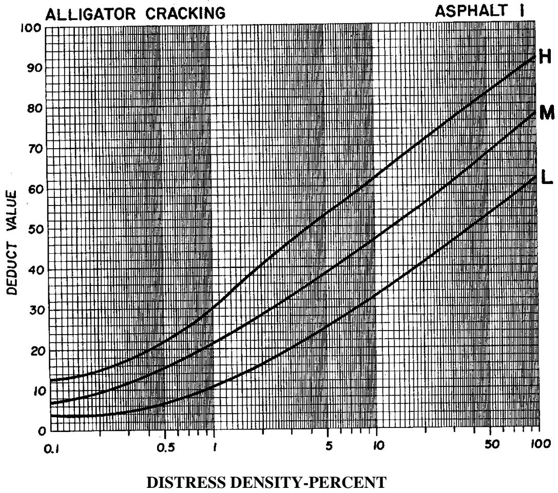
Lampiran 1. Grafik PCI Deduct Value Alligator Cracking
