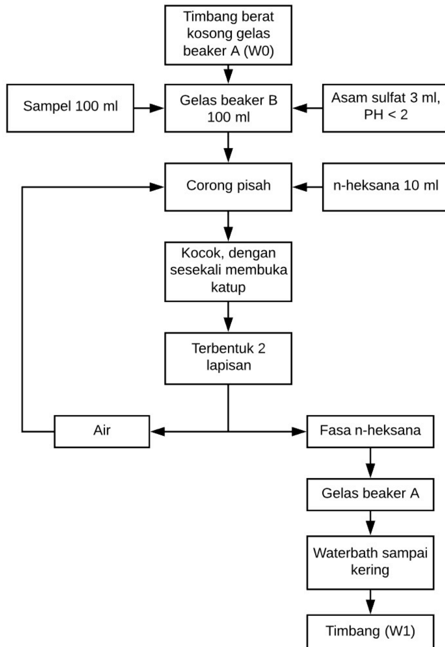
Diagram Alir Pengujian Oil and Grease
