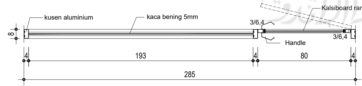
POT. 3-3 skala 1: 20
