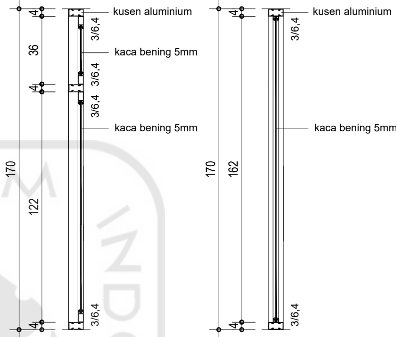
POT. 16-16 skala 1: 20 POT. 16a-16a skala 1: 20 DETAIL J1 Skala 1 : 20
