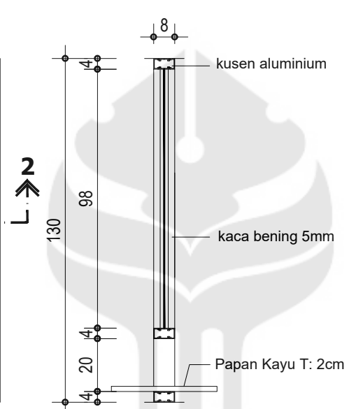
POT. 1-1 skala 1: 20
