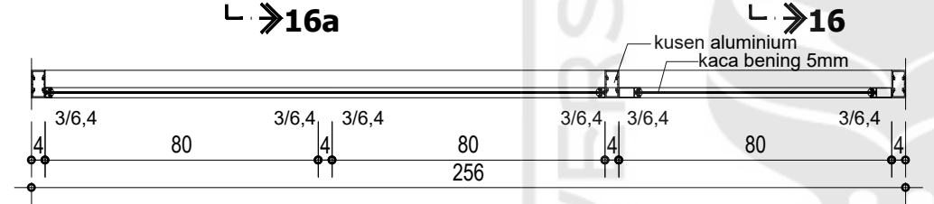
POT. 17-17 skala 1: 20
