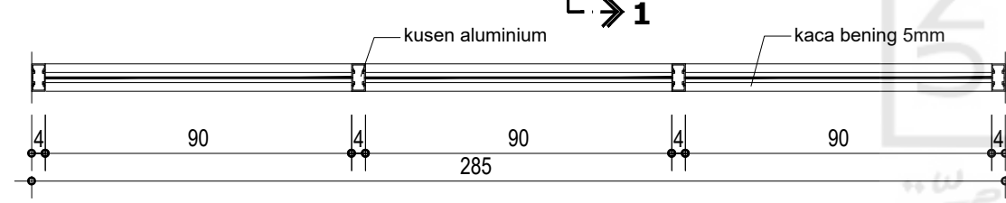
POT. 2-2 skala 1: 20
