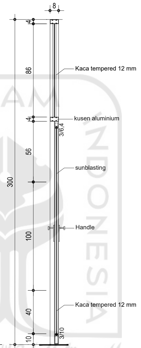
POT. 1-1 skala 1: 20
