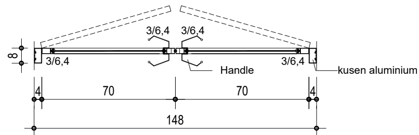
POT. 4-4 skala 1: 20
