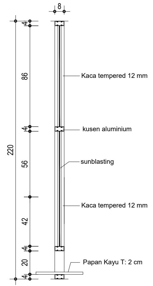
POT. 2-2 skala 1: 20
