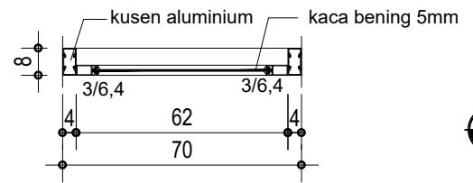
POT. 19-19 skala 1: 20
