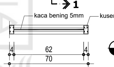
POT. 2-2 skala 1: 20
