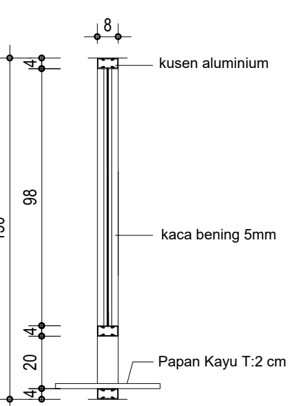
POT. 1-1 skala 1: 20
