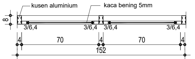
POT. 21-21 skala 1: 20
