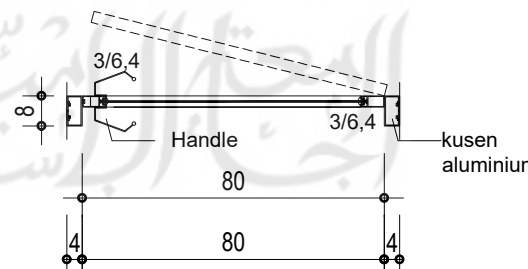
POT. 6-6 skala 1: 20
