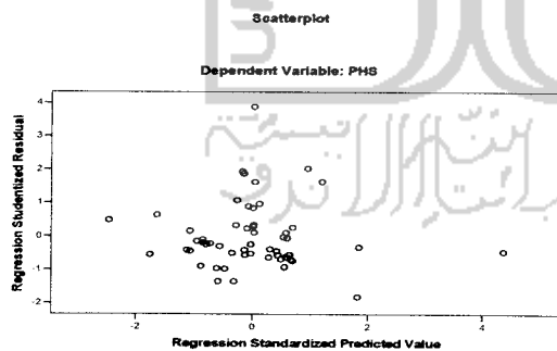
Gambar 4.3.4.1 Scatterplot
