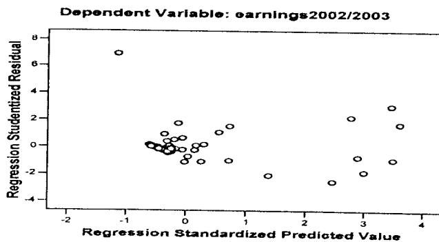
Scatterplot
