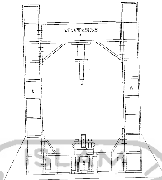
Gambar 4.11 Loading Frame
