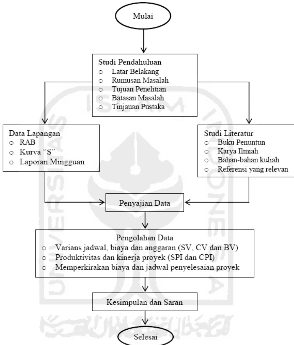
Gambar 4.1 Flowchart Penelitian
