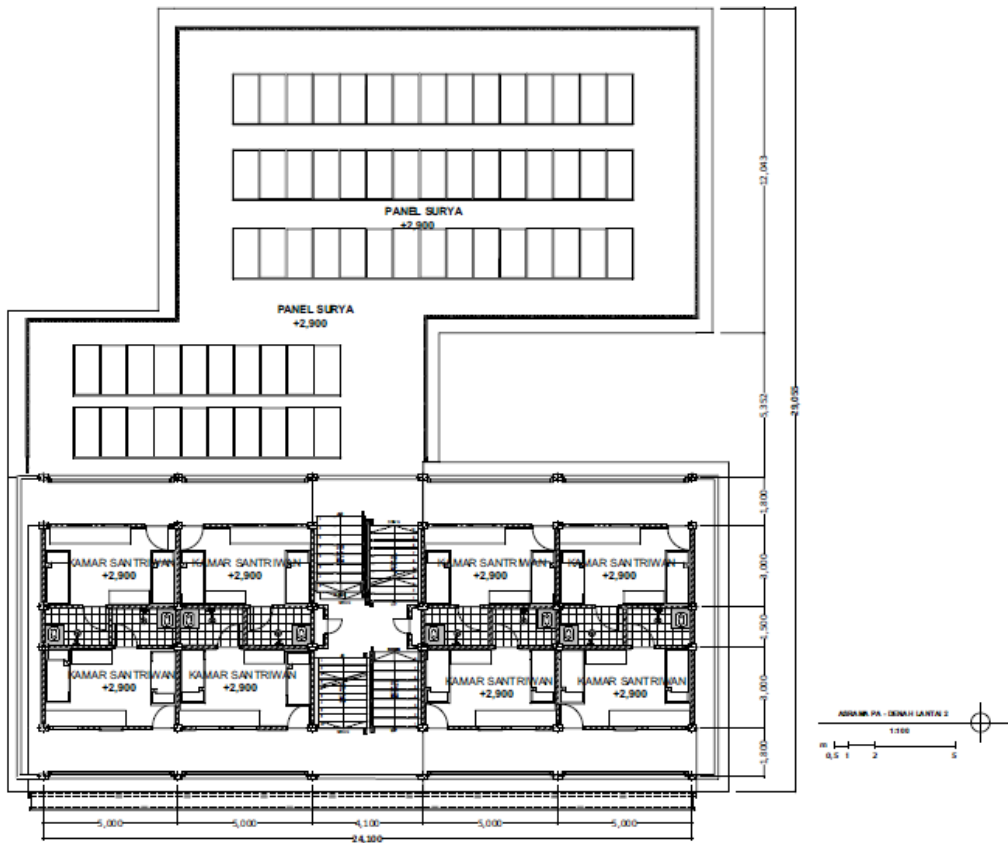
Denah Asrama Santriwan lantai 2
