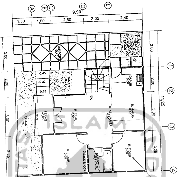
DENAH LANTAI 01
