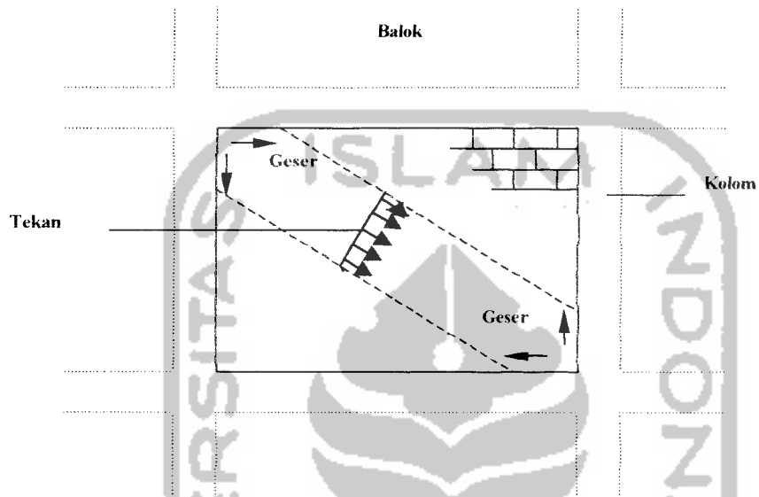
Gambar 3.5 Gambar Distribusi Beban Geser
