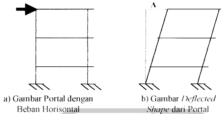
Gambar 3.3 Gambar Deflected Shape
