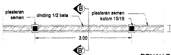
DENAH PAGAR2 1:25
