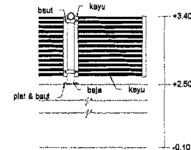
DETAIL R2 1:25
