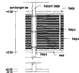
DETAIL R1 1:25
