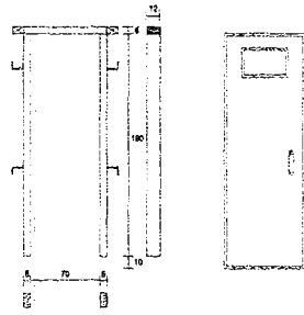
DETAIL P4
