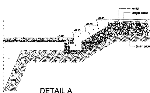
DETAIL A 1:20
