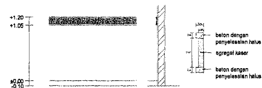
DETAIL R3 1:25
