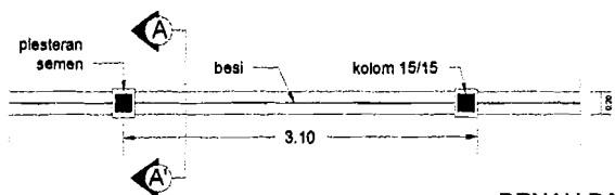
DENAH PAGAR1 1:25
