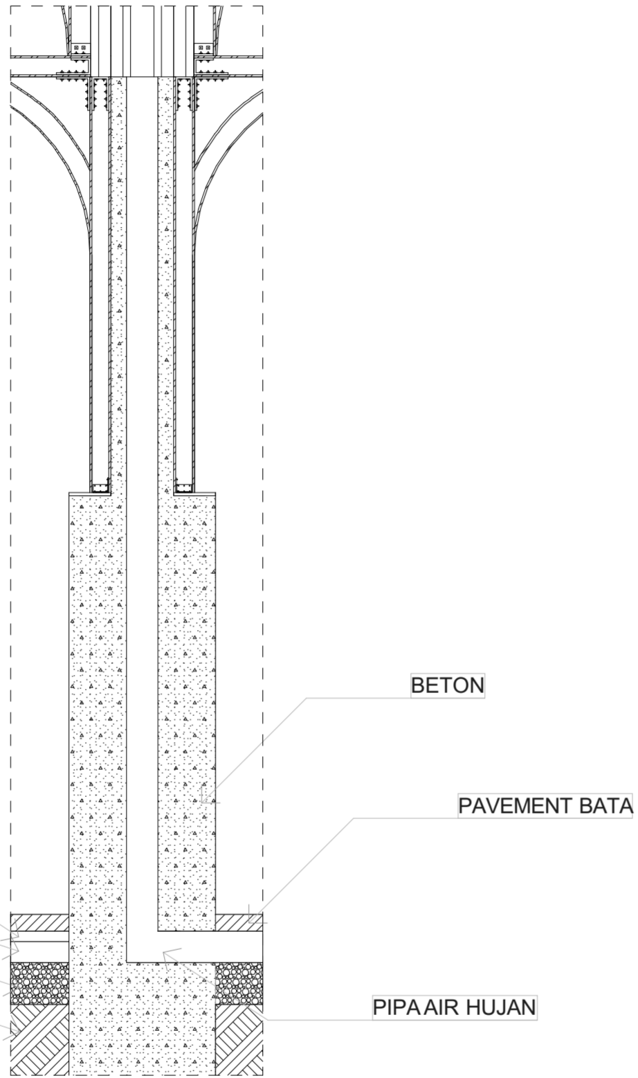
D-04 Detail 1:25
