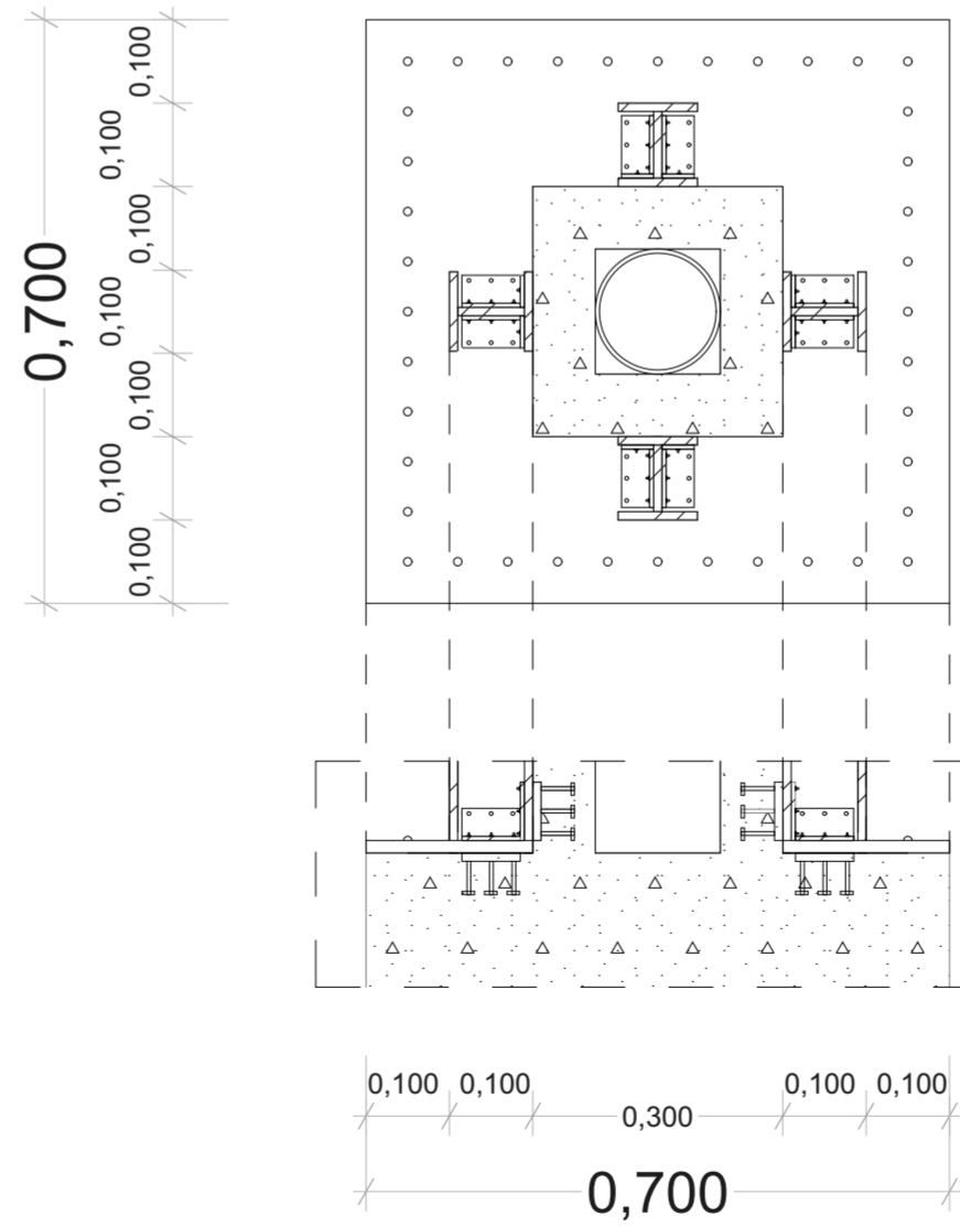
D-06 Detail 1:10
