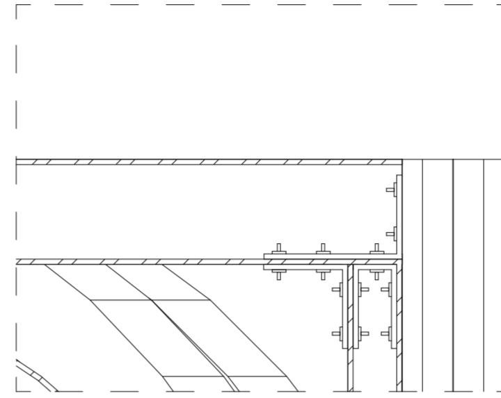
D-05 Detail 1:10
