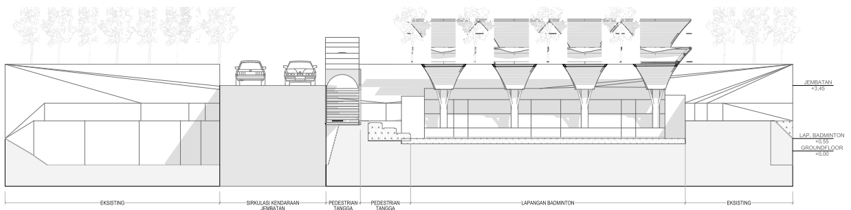
POTONGAN PARSIAL BADMINTON 1/100
