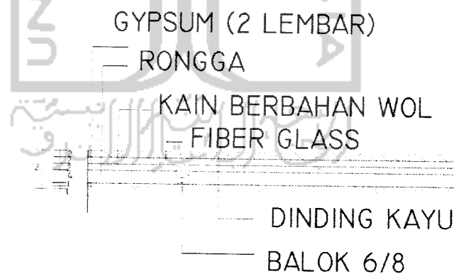
Gambar 6.2 Rekomendasi Detail Dinding
