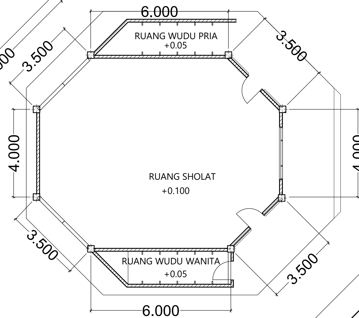
DENAH MUSHOLA 1:100
