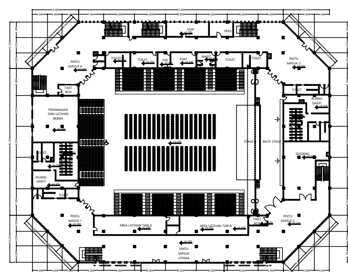
KEY PLAN 1:1000
